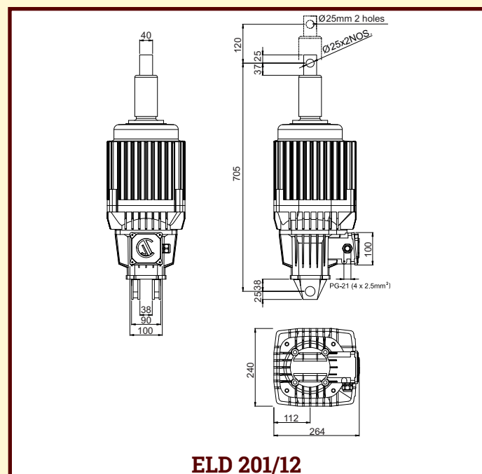
ELECTRO-HYDRAULIC THRUSTER MODEL ELD 201/12
