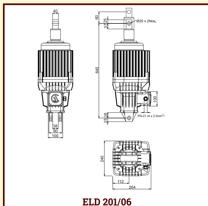
ELECTRO-HYDRAULIC THRUSTER MODEL ELD 201/06
