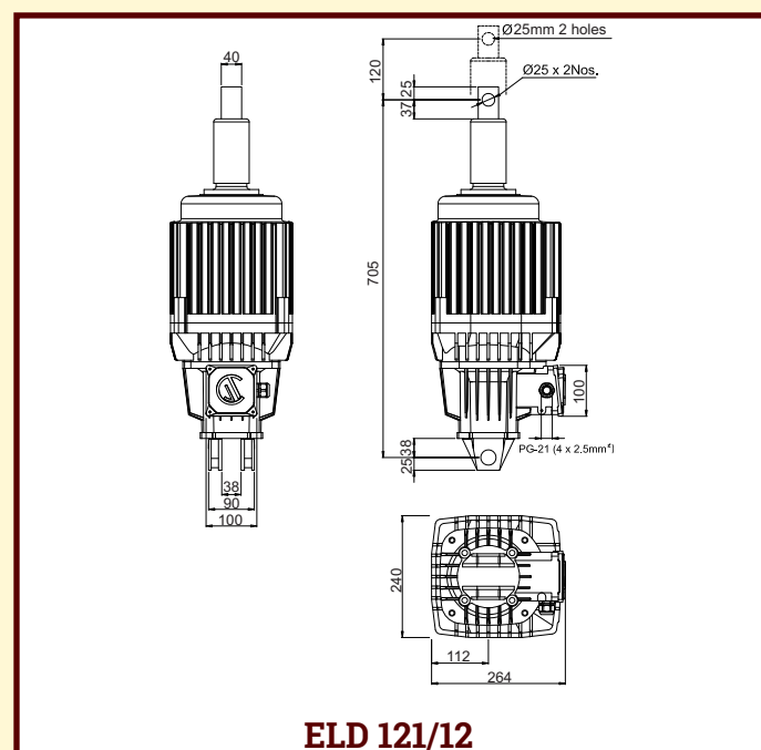
ELECTRO-HYDRAULIC THRUSTER MODEL ELD 121/12
