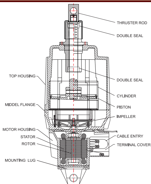
SECTIONAL VIEW
