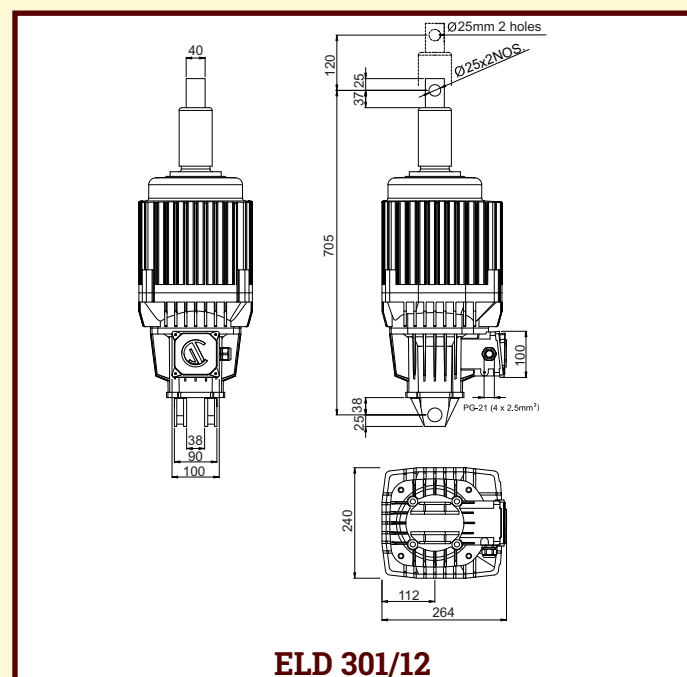
ELECTRO-HYDRAULIC THRUSTER MODEL ELD 301/12
