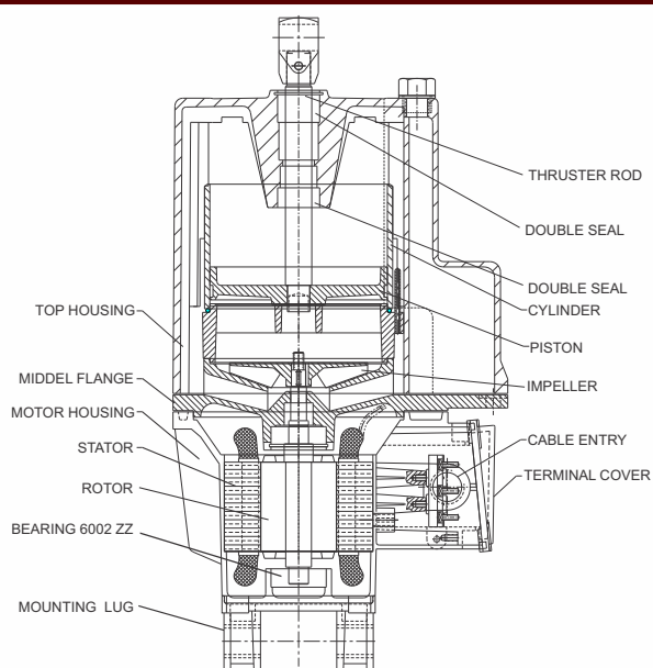
SECTIONAL VIEW
