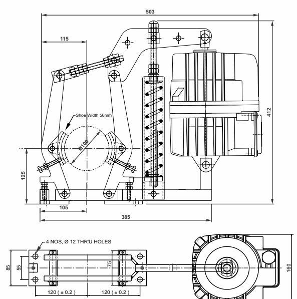
SMD-100-23/5-LAF
