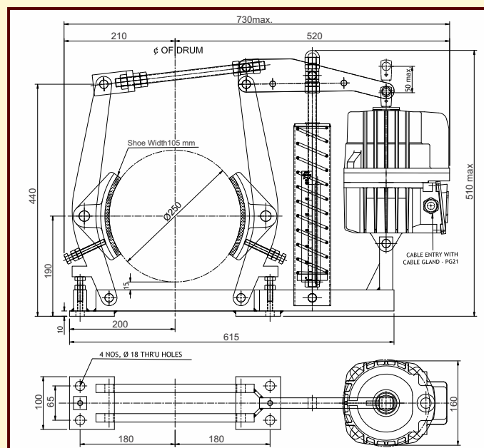
SMD-250-23/5-LAF
