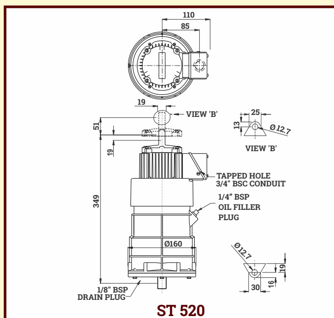
ELECTRO-HYDRAULIC THRUSTER MODEL ST 520
