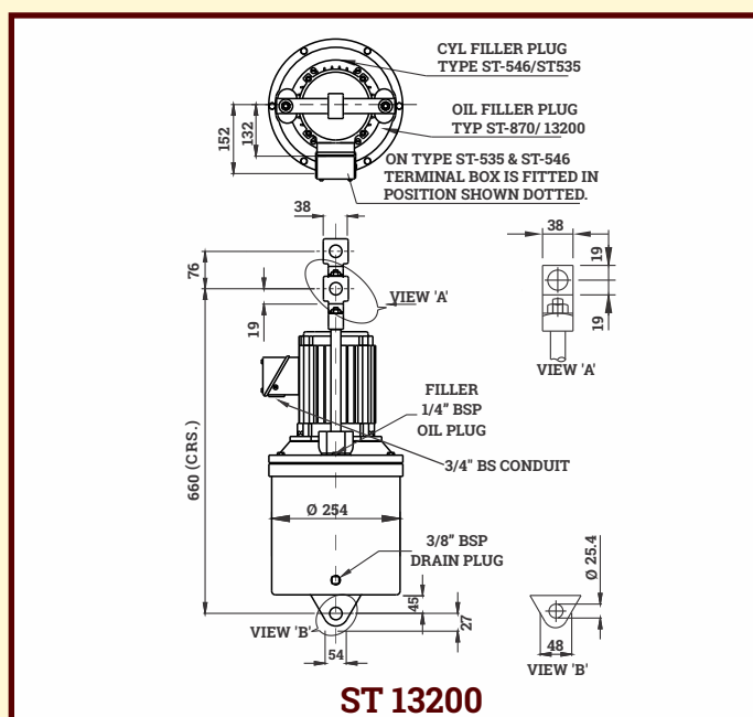
ELECTRO-HYDRAULIC THRUSTER MODEL ST 13200
